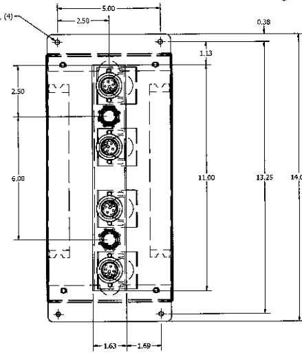
MODEL DC14-4-120
